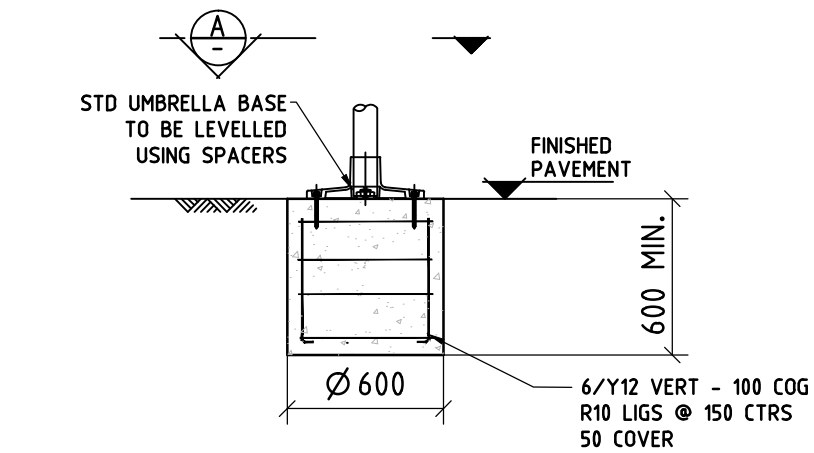
FOOTING OPTION A - BORED PIER
