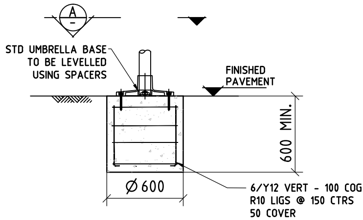
FOOTING OPTION A - BORED PIER
