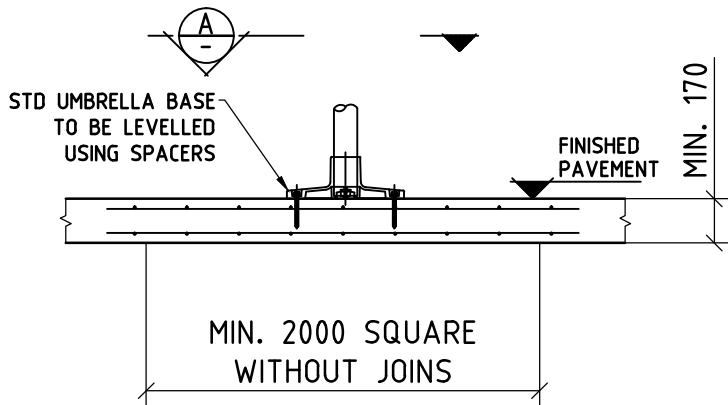
FOOTING OPTION B - PAD FOOTING
