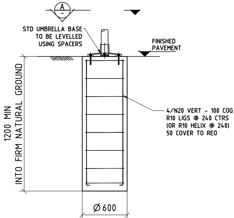
FOOTING OPTION A - BORED PIER
