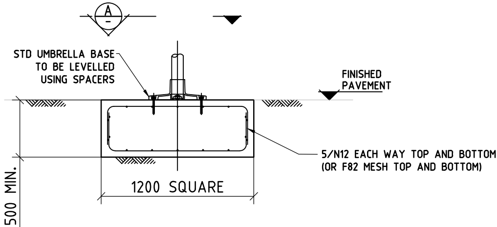
FOOTING OPTION B - PAD FOOTING
