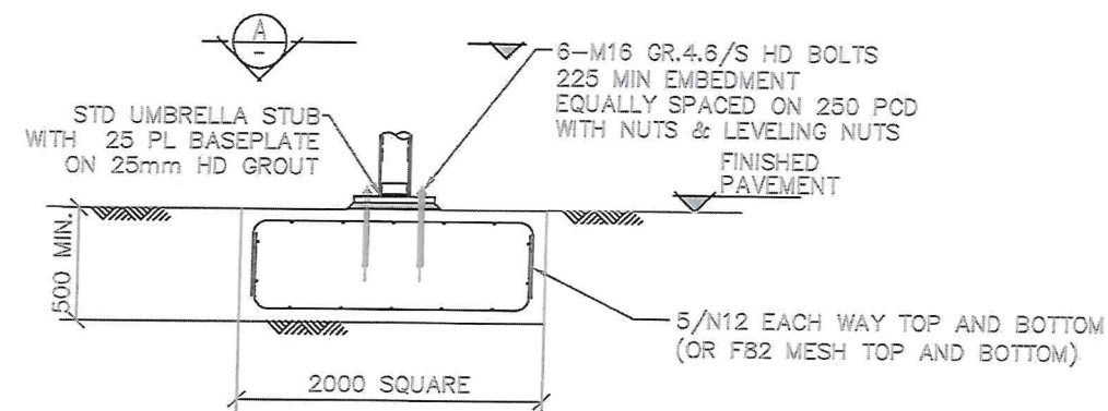
FOOTING OPTION B - PAD FOOTING
