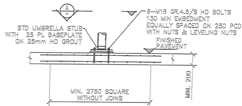
FOOTING OPTION C - EXISTING SLAB
