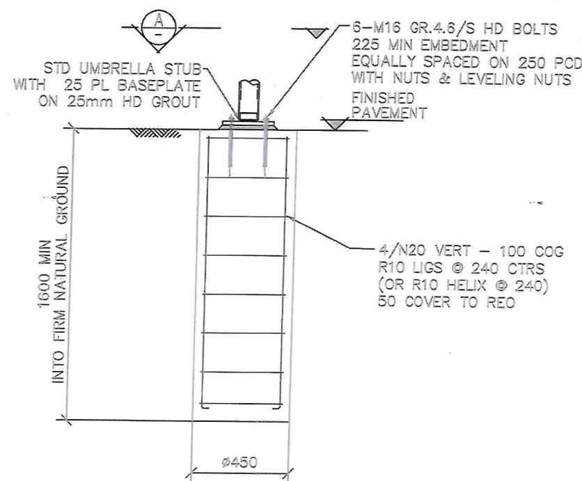
FOOTING OPTION A - BORED PIER
